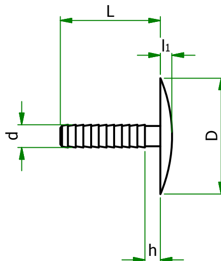
Male Clip
