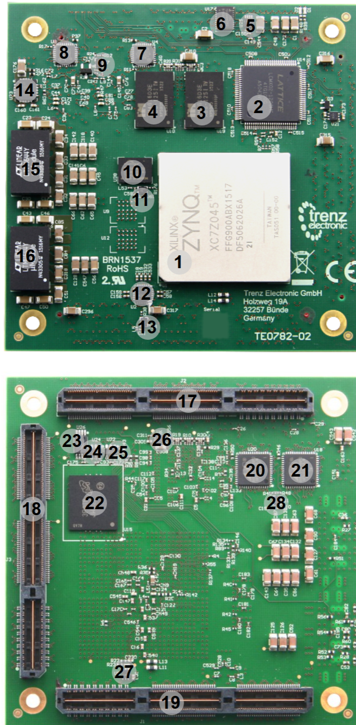
Figure 2: TE0782-02 main components
