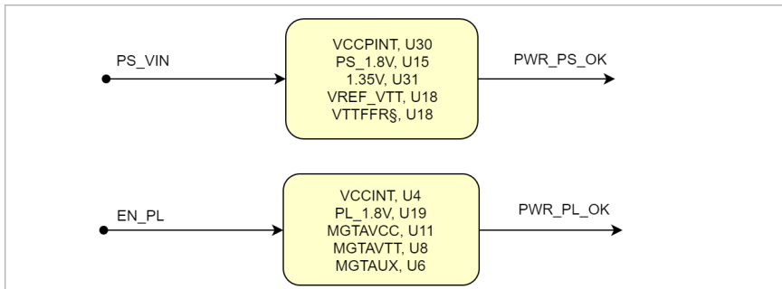
Figure 4: Power Sequency
