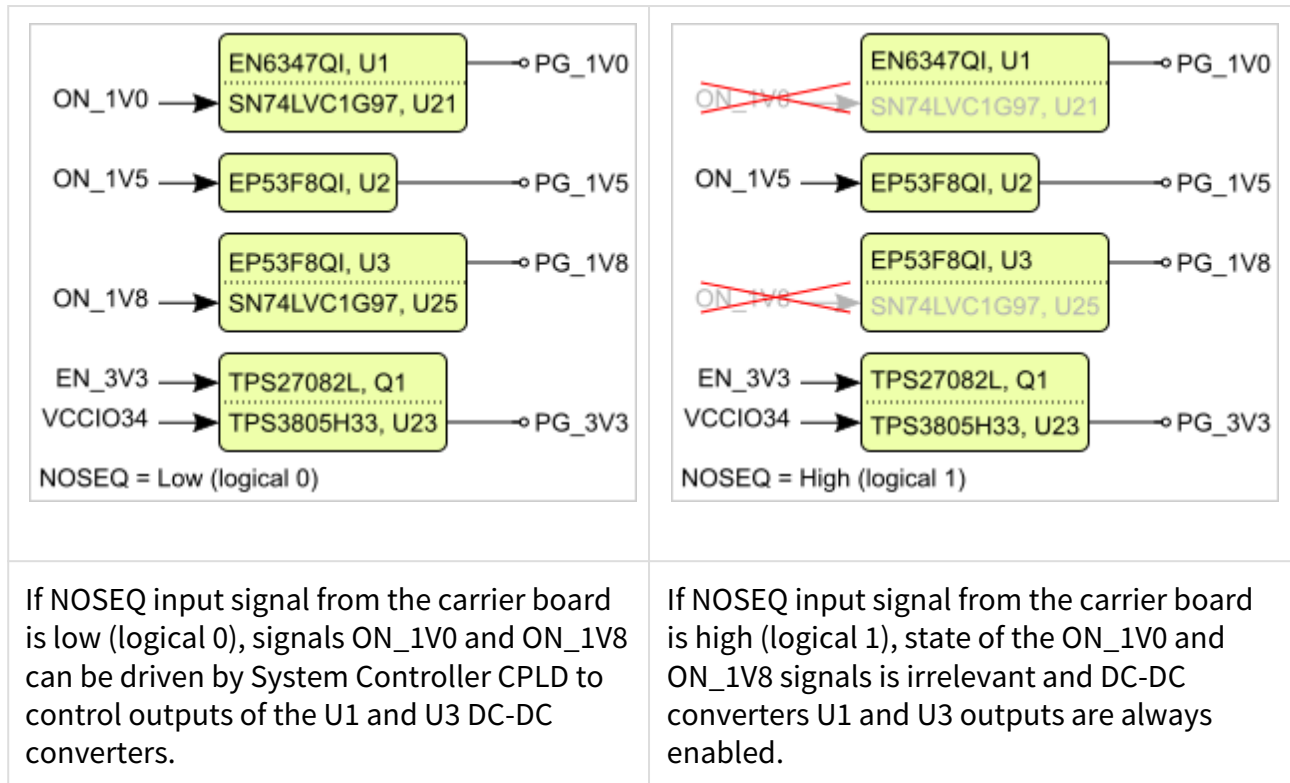
Figure 4: Power sequencing.
