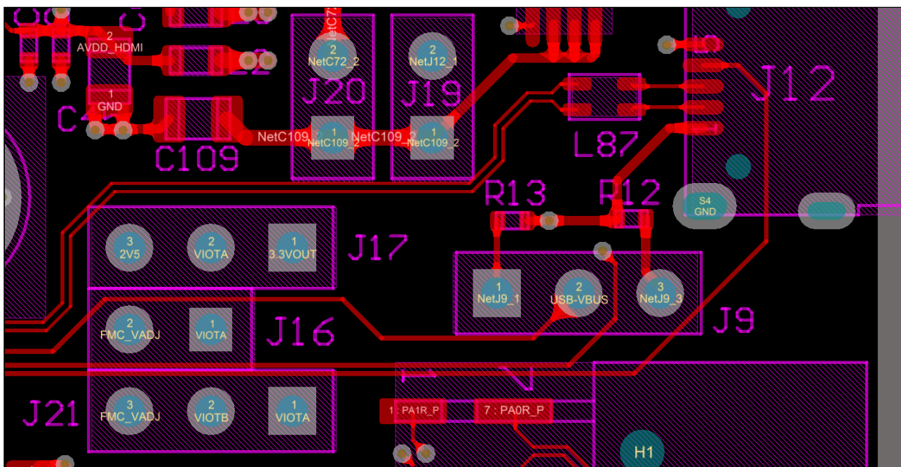
Figure 7: VCCIO jumper pin location (PCB-REV06), top view
