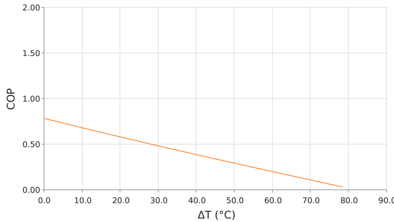
Coefficient of Performance (COP = Q_c/P_{in} ) T_{hot} = 50^\circ\text{C} | I_{operating} = 10.4 Amps
