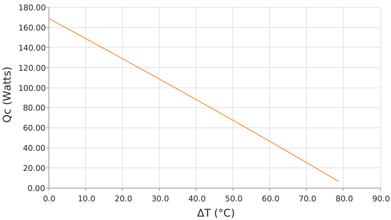
Heat Pumped at Cold Side ( Q_c ) T_{hot} = 50^\circ\text{C} | I_{operating} = 10.4 Amps
