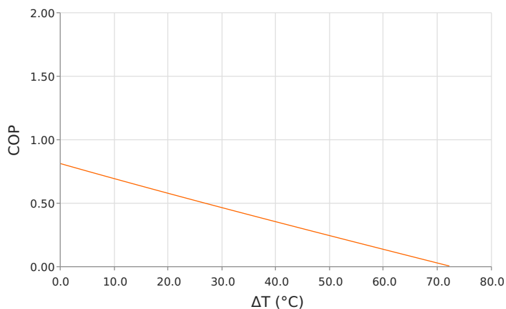
Coefficient of Performance (COP = Q_c/P_{in} ) T_{hot} = 27\text{ }^{\circ}\text{C} | Current = 8.7 Amps
