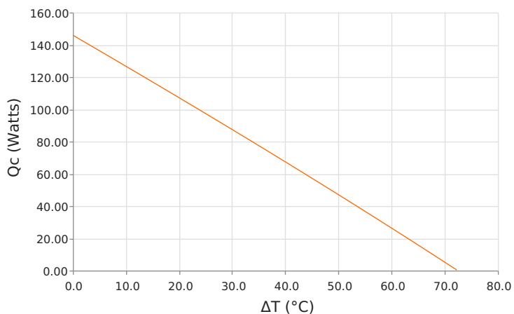
Heat Pumped at Cold Side ( Q_c ) T_{hot} = 27\text{ }^{\circ}\text{C} | Current = 8.7 Amps
