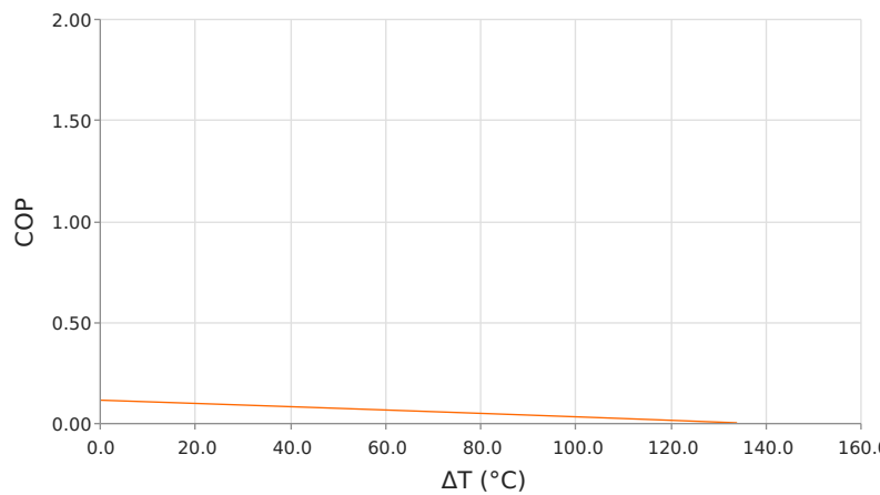
Coefficient of Performance (COP = Q_c/P_{in} ) T_{hot} = 35\text{ }^{\circ}\text{C} | operating = 1.4 Amps
