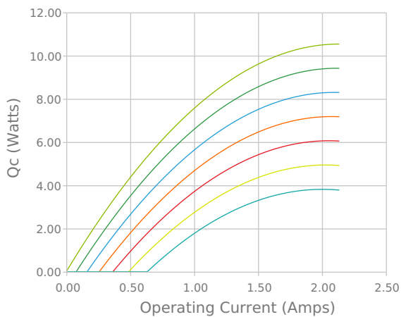
Heat Pumped at Cold Side T_{hot} = 85^\circ C
