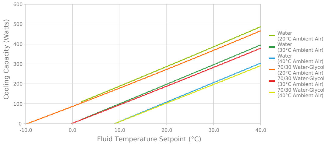
MRC300-DH2-HT-DV \Delta T (Inlet-Outlet) Fluid Temperature
