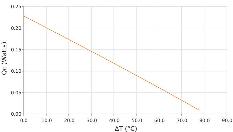
Heat Pumped at Cold Side (Qc) Thot = 50 °C | Ioperating = 0.7 Amps
