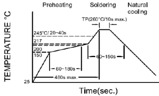
Figure 1. : Re-flow Soldering time 3 times Max.
