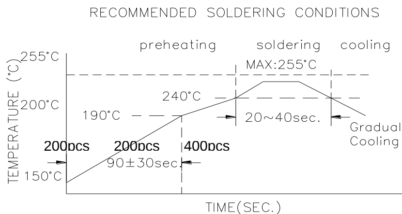
Figure 1 . Re-flow Soldering
