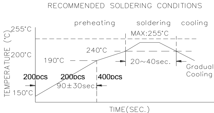
Figure 1 . Re-flow Soldering
