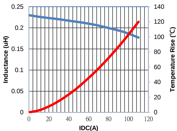
MGV1205R22M-10
