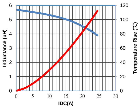
MGV12055R6M-10
