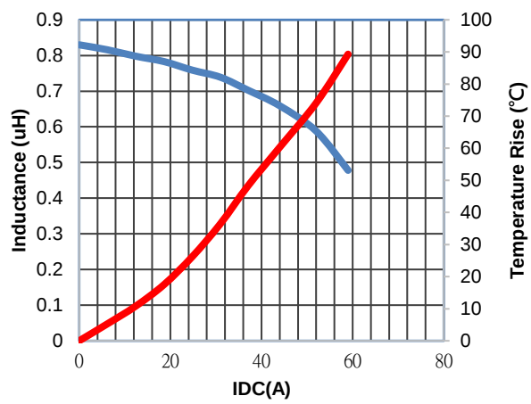
MGV1205R82M-10
