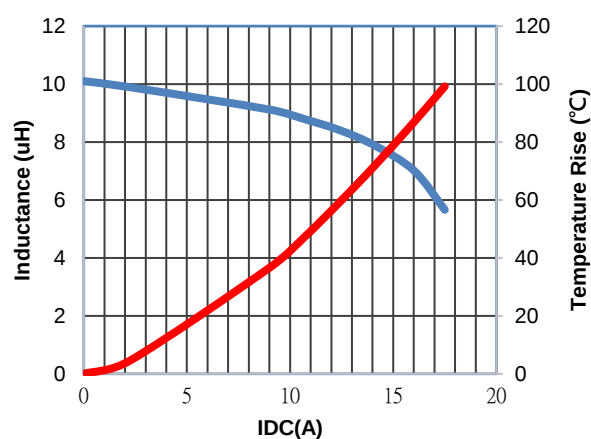
MGV1205100M-10
