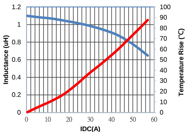
MGV12051R0M-10
