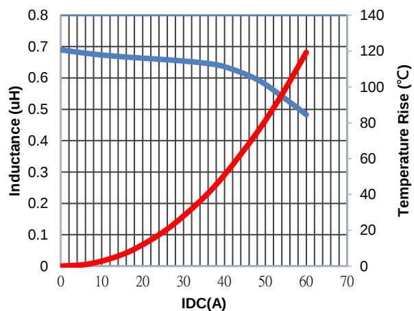
MGV1205R68M-10
