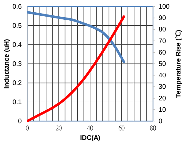
MGV1205R56M-10
