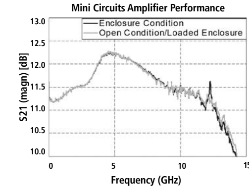
Figure 6. Performance in Enclosure and Using Foam Absorber
