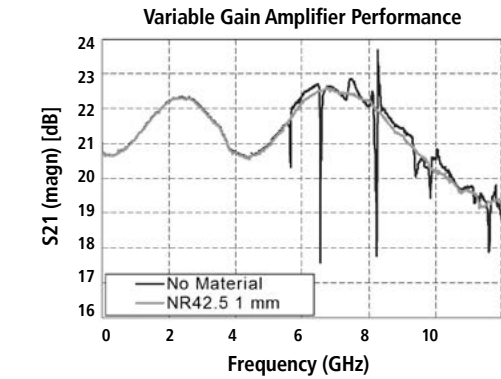
Figure 4. Performance of amplifier inside enclosure showing performance of Absorber Material (PN 2238)
