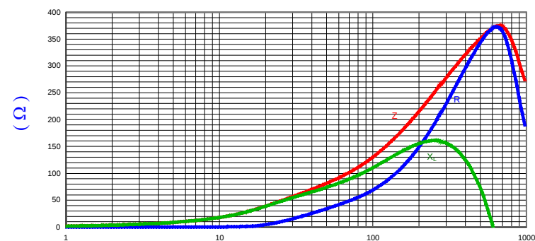
NET Z,R AND X vs. FREQUENCY
