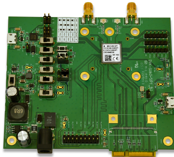
Figure 1: Development board
