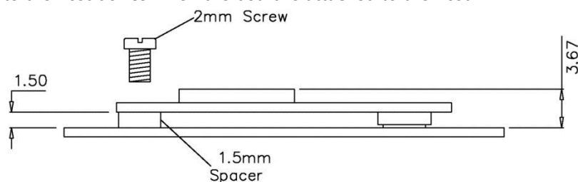
Figure 7: Mounting Recommendations
