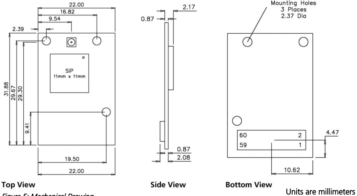
Figure 5: Mechanical Drawing
