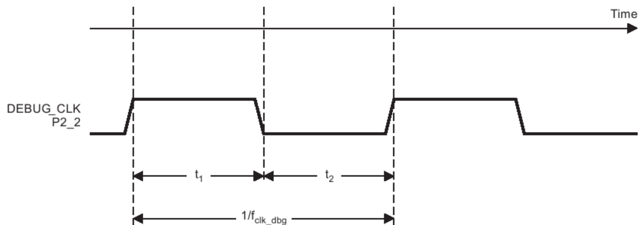
Figure 5 Slave Timing
