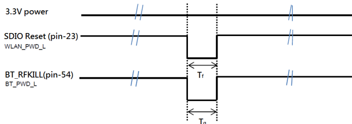
Figure 3: Reset Timing
