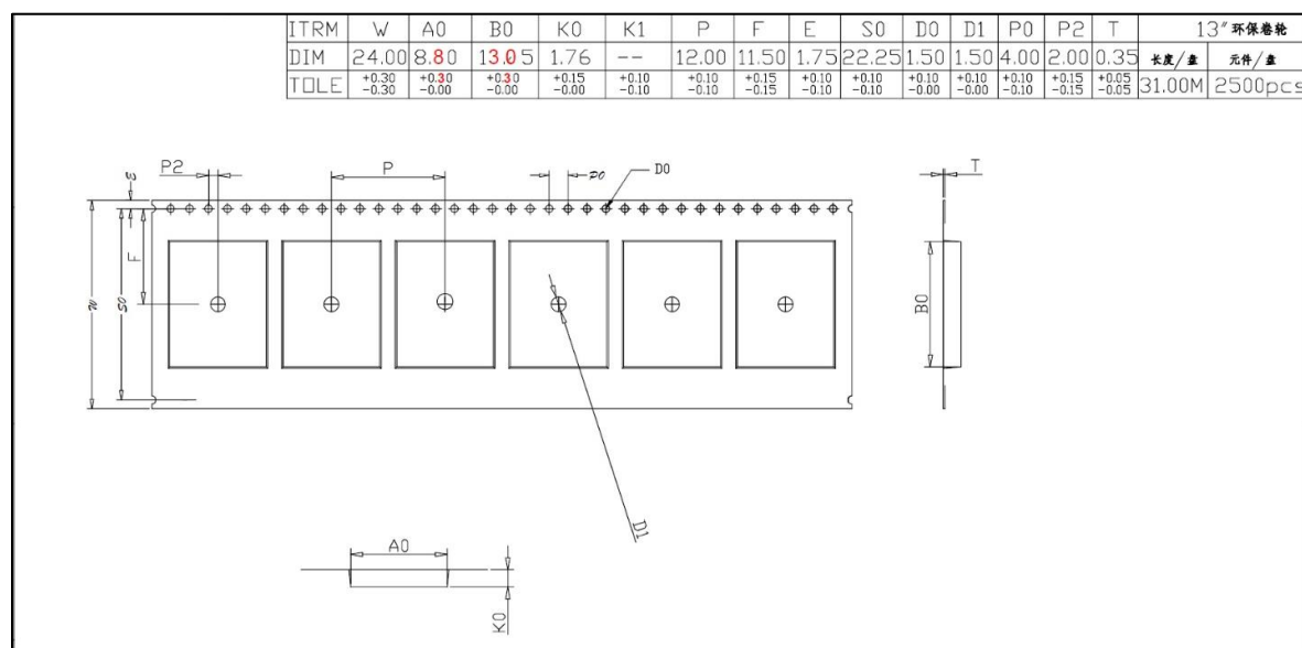
Figure 23: Tape specifications
