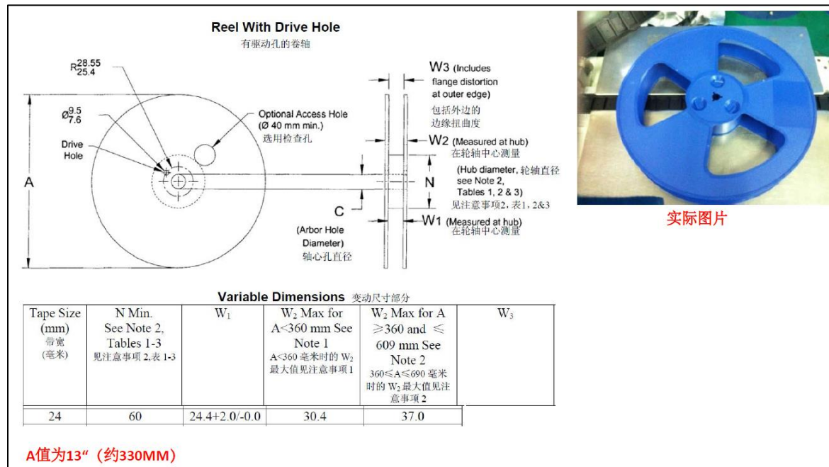
Figure 22: Reel specifications
