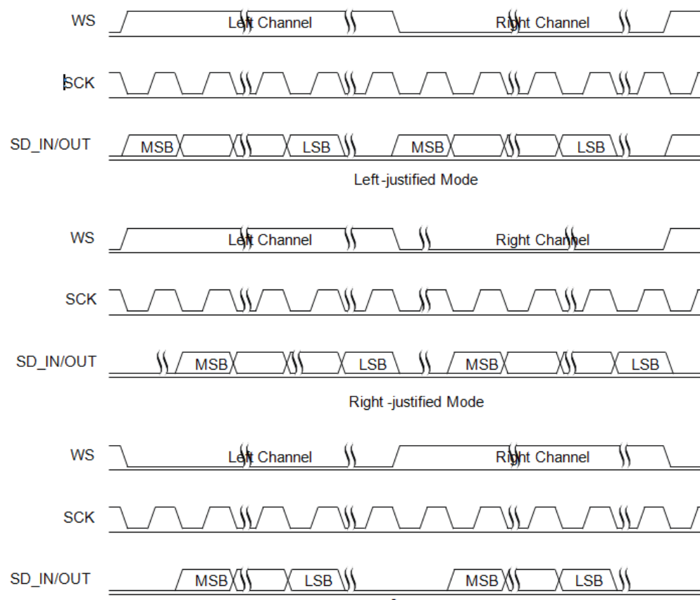
Figure 13: PCM configuration
