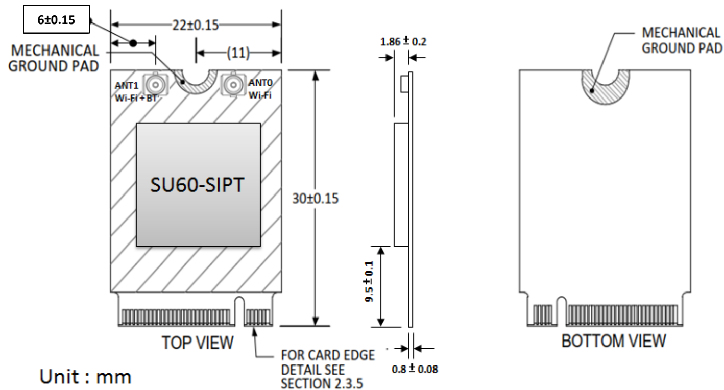
Figure 8: Module dimension of 60-2230C
