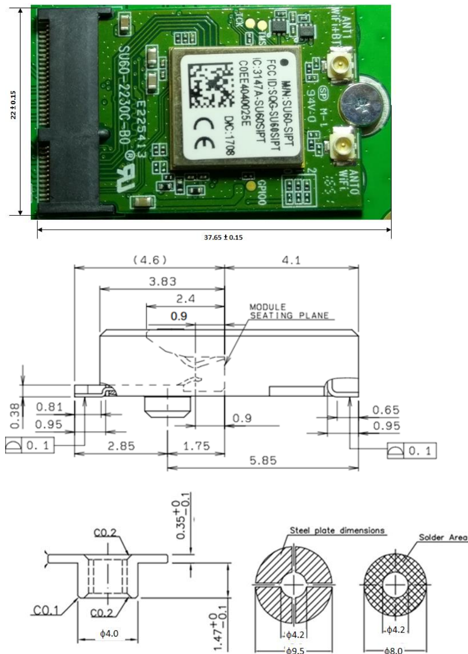
Figure 9: Mounting information of the 60-2230C and recommended layout pattern for the stand-off
