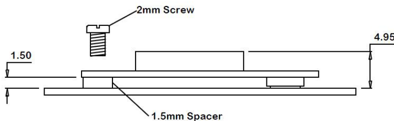
Figure 11: Mounting Recommendations
