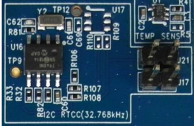
Figure 16: I2C device RTC chip schematic and PCB
