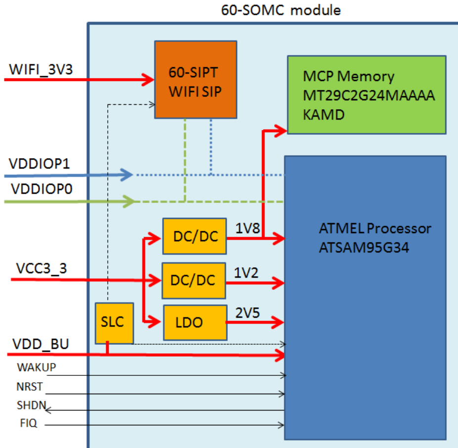
Figure 2: 60-SOM module power supply
