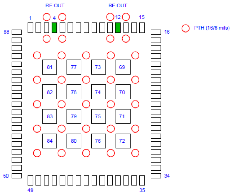
Figure 12: Recommended ground via
