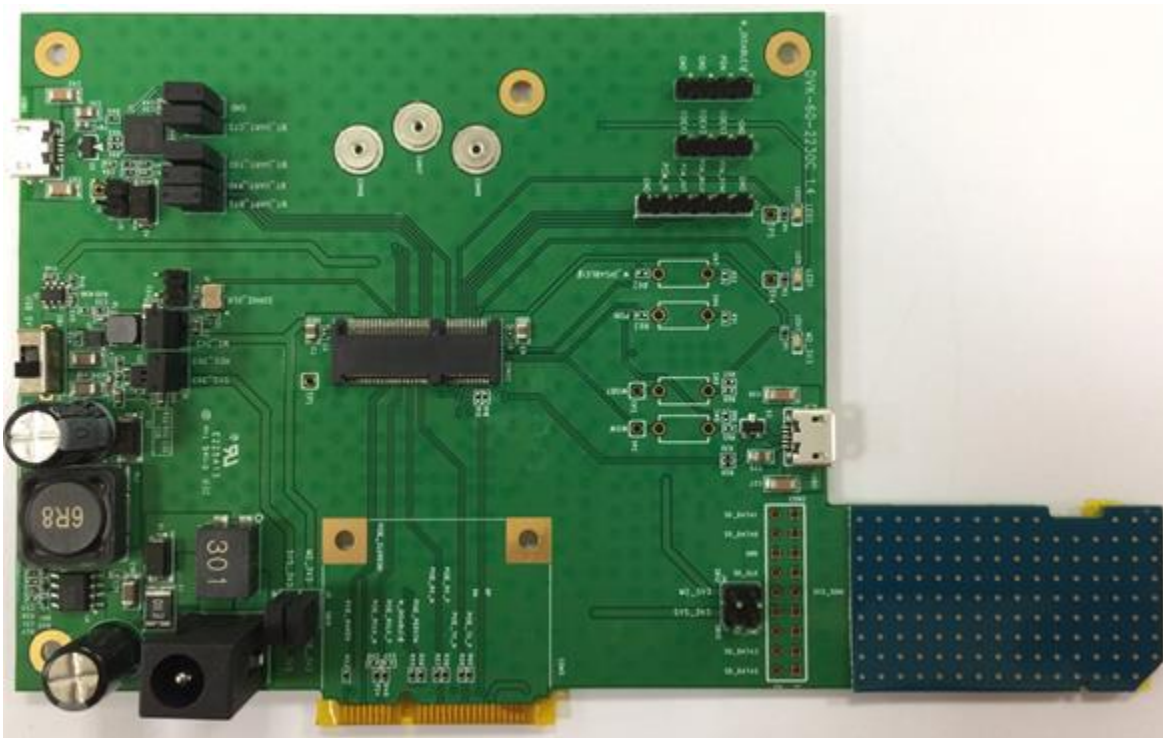
Figure 1: Development board
