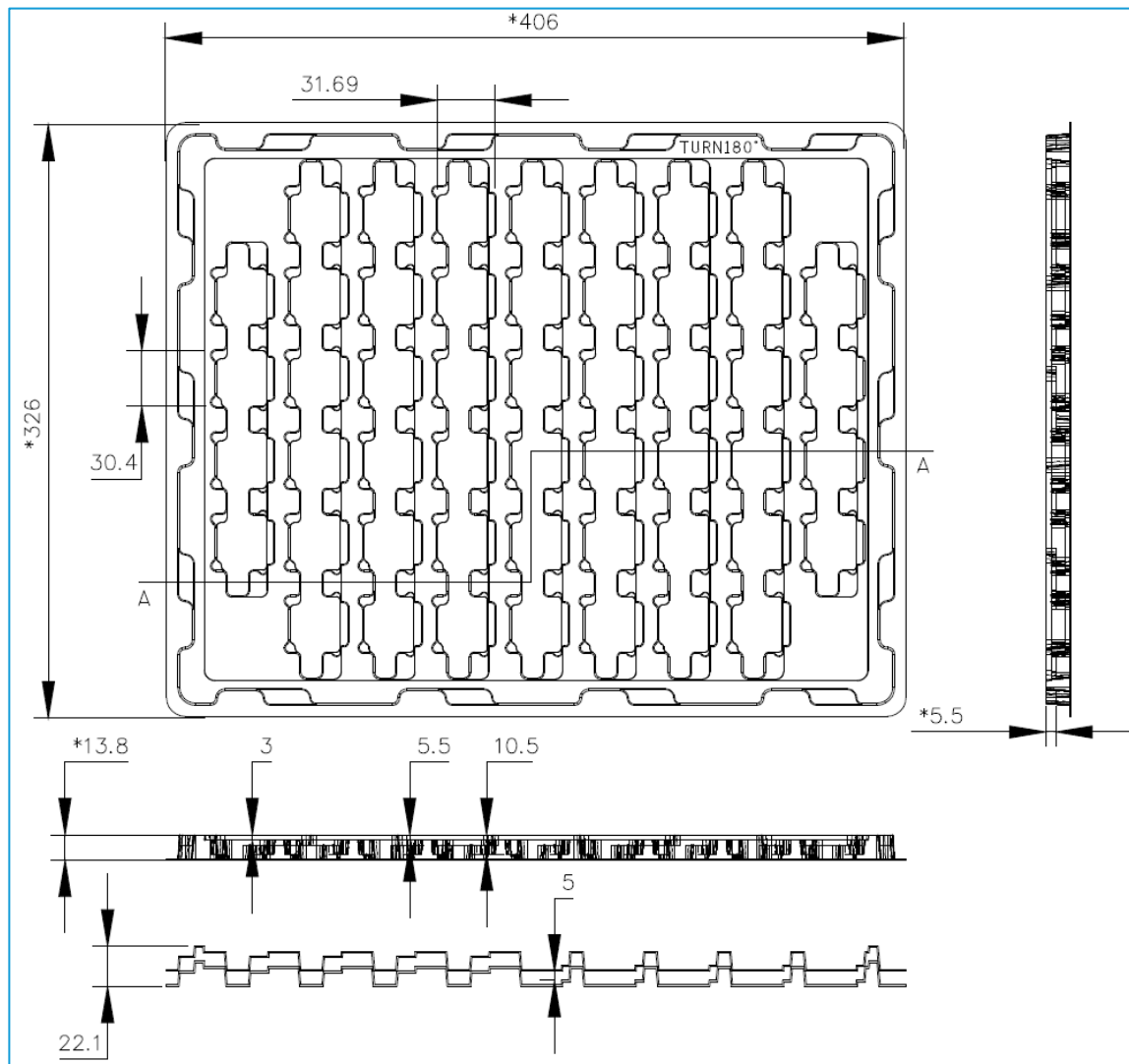
Figure 10: 453-00011 modem tray (mm) 50 per tray
