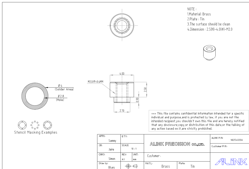
Figure 7: PEM Threaded Standoff mechanical drawings
