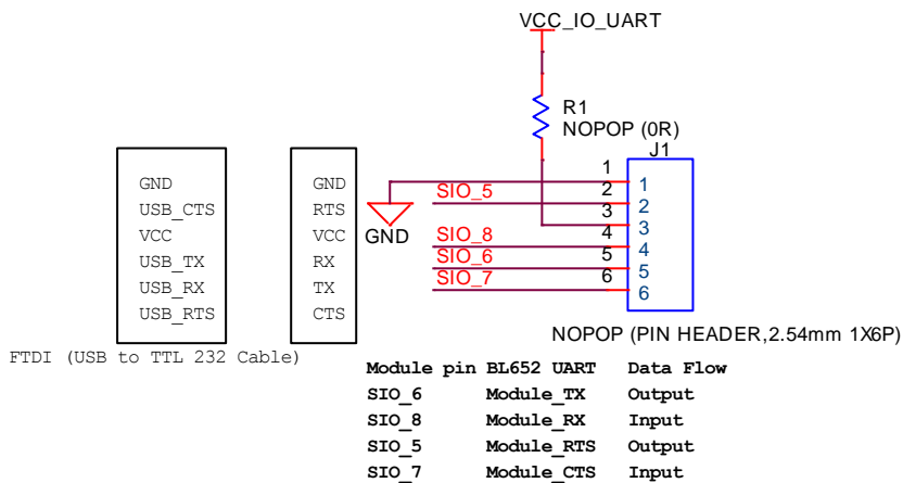
Figure 9: J1 wiring to match FTDI USB-UART cable (TTL-232R-3V3 cable)
