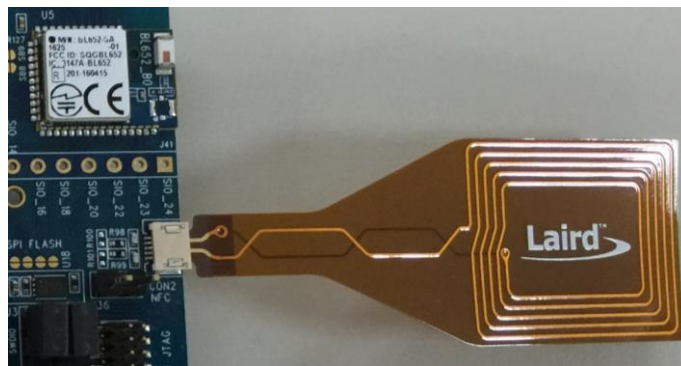
Figure 16: NFC antenna RF matching circuit, NFC antenna connector schematic and NFC plugged in to connector CON2
