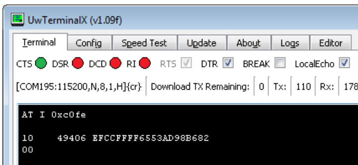
Figure 8: AT+I0xc0fe command returning the module license
