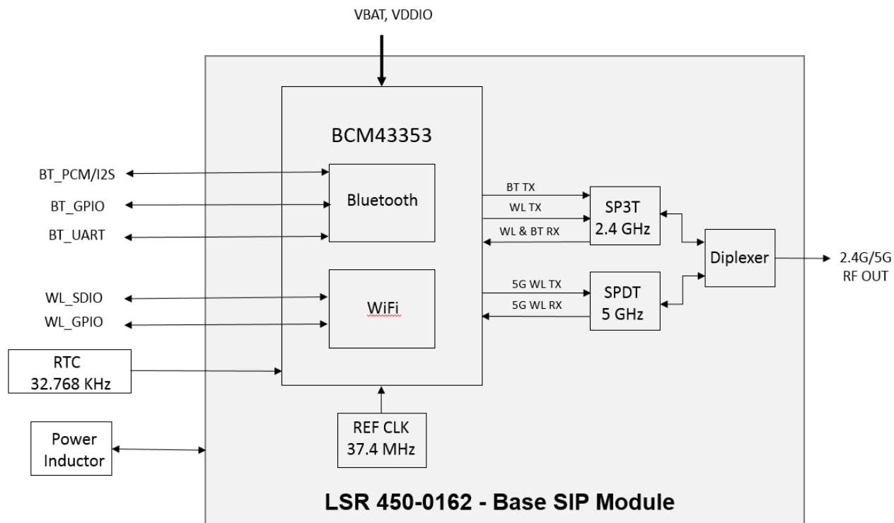
Figure 4 Sterling-LWB5 Base SIP Module Block Diagram
