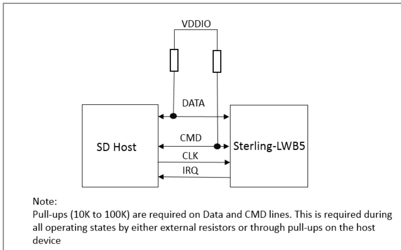
Figure 18 Signal Connections to SDIO Host (SD 1-Bit Mode)
