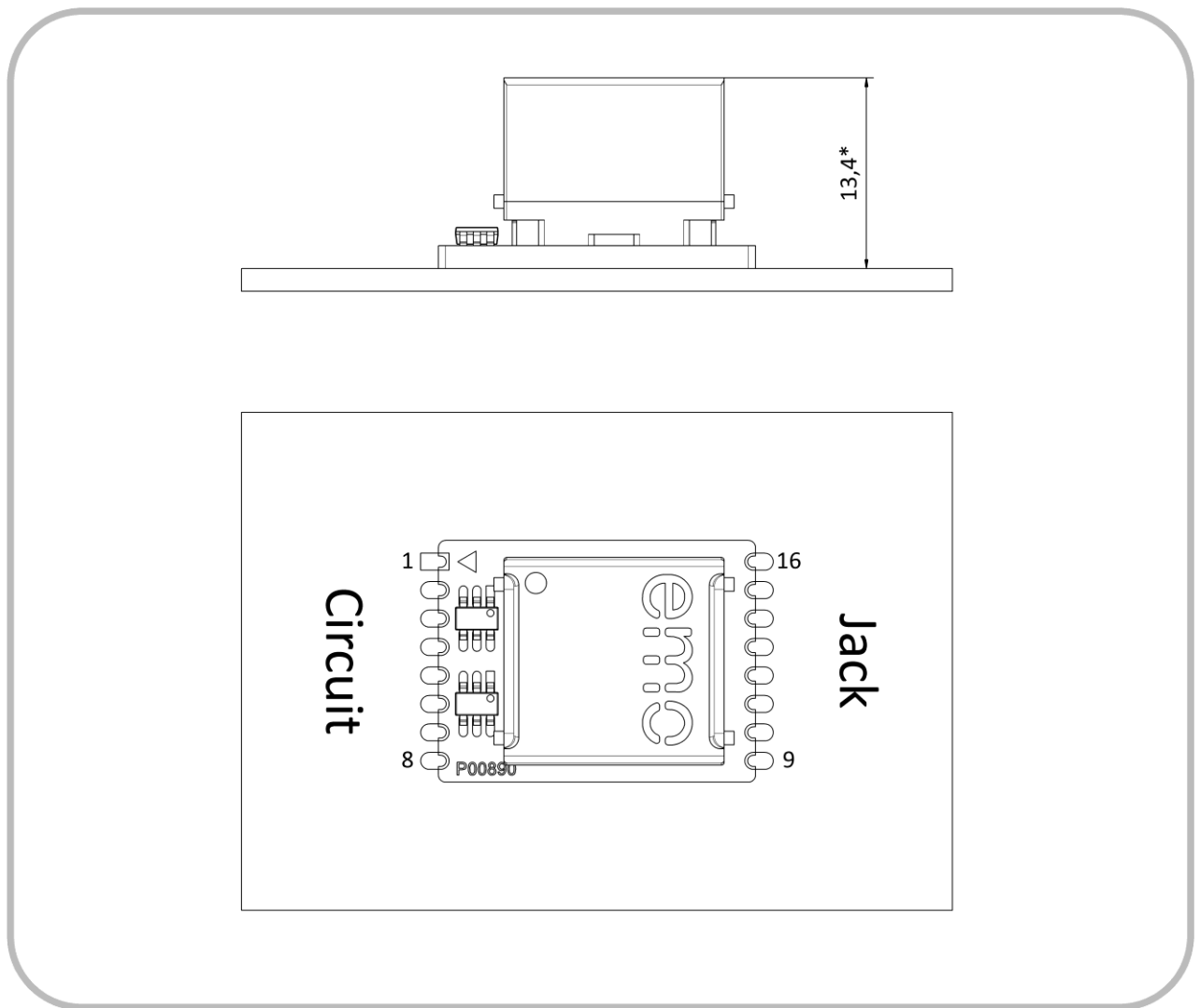
Figure 8. Physical dimensions of an EN-100S assembled onto a PCB. The labels Jack and Circuit indicate the intended locations of the RJ45 Ethernet Jack and the product circuitry, respectively.
