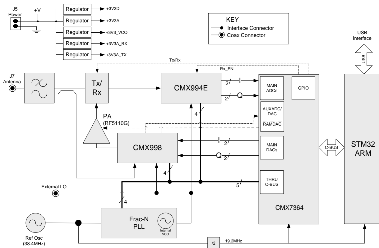
Figure 1 Block Diagram
