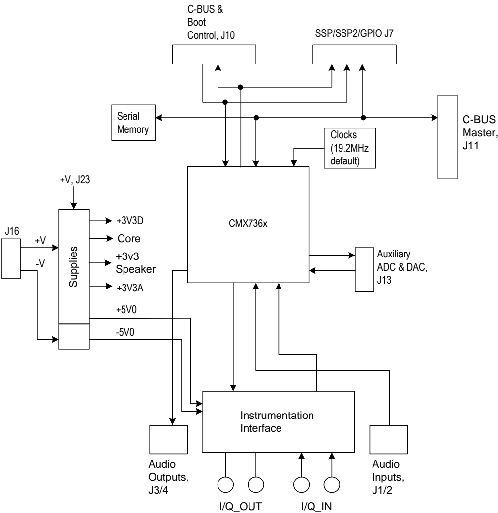
Figure 1 Block Diagram
