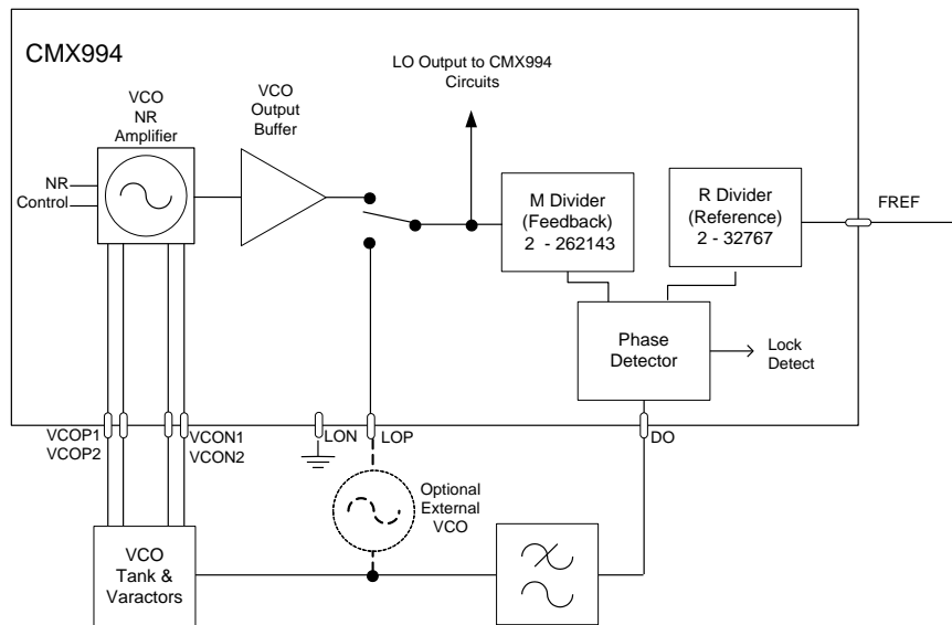
Figure 16 Local Oscillator
