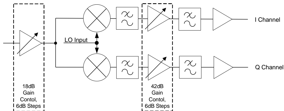
Figure 22 Gain Control
