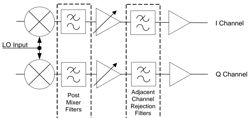
Figure 14 Baseband I/Q Filtering
