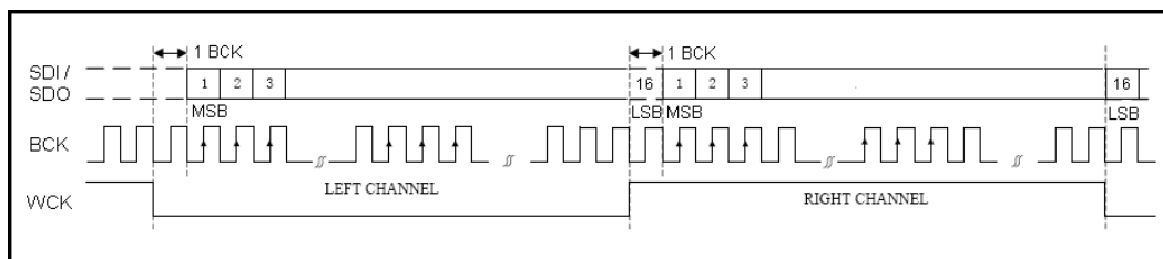
Figure 8-1 I2S Interface Data Format
