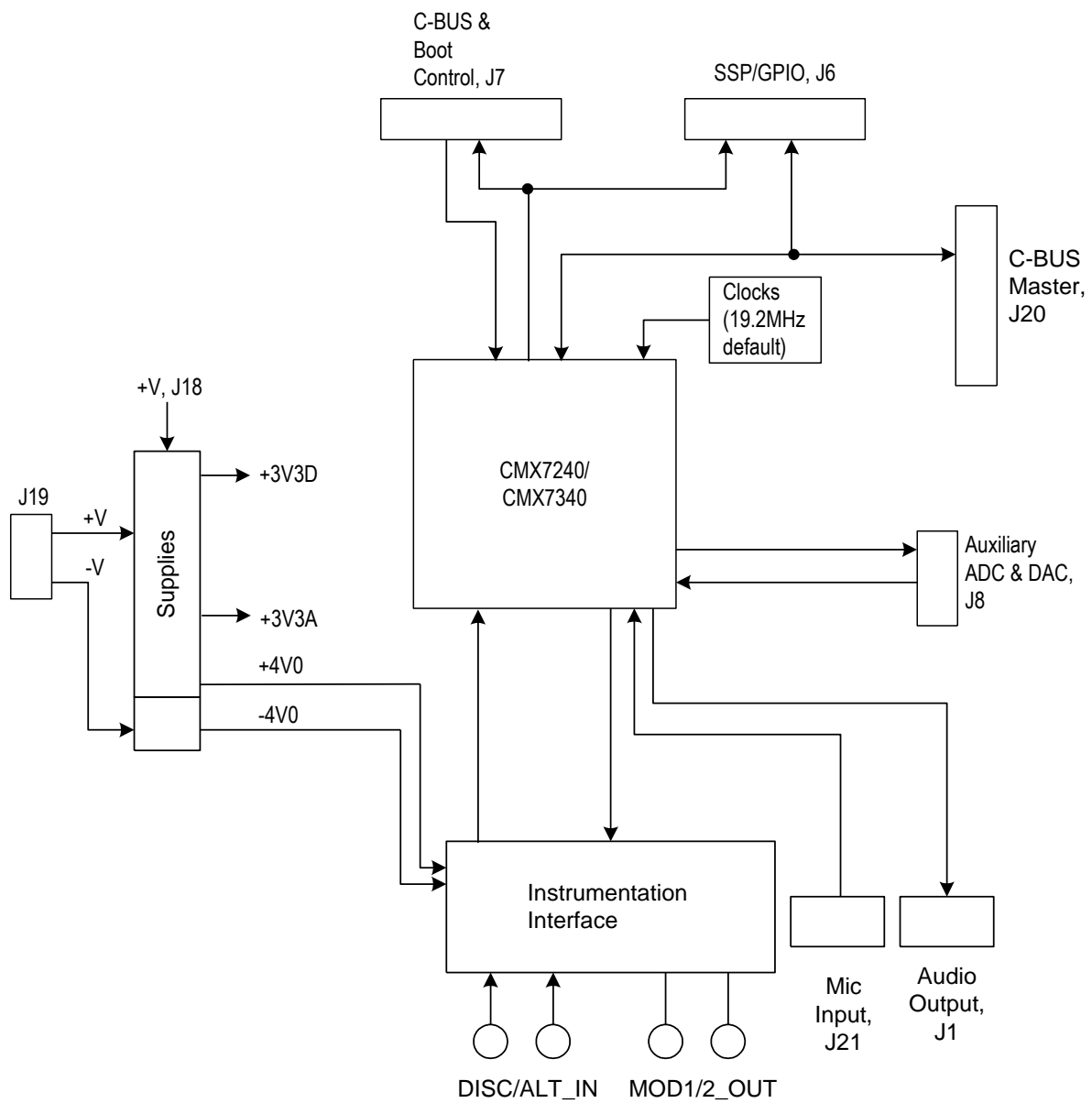
Figure 1 Block Diagram
