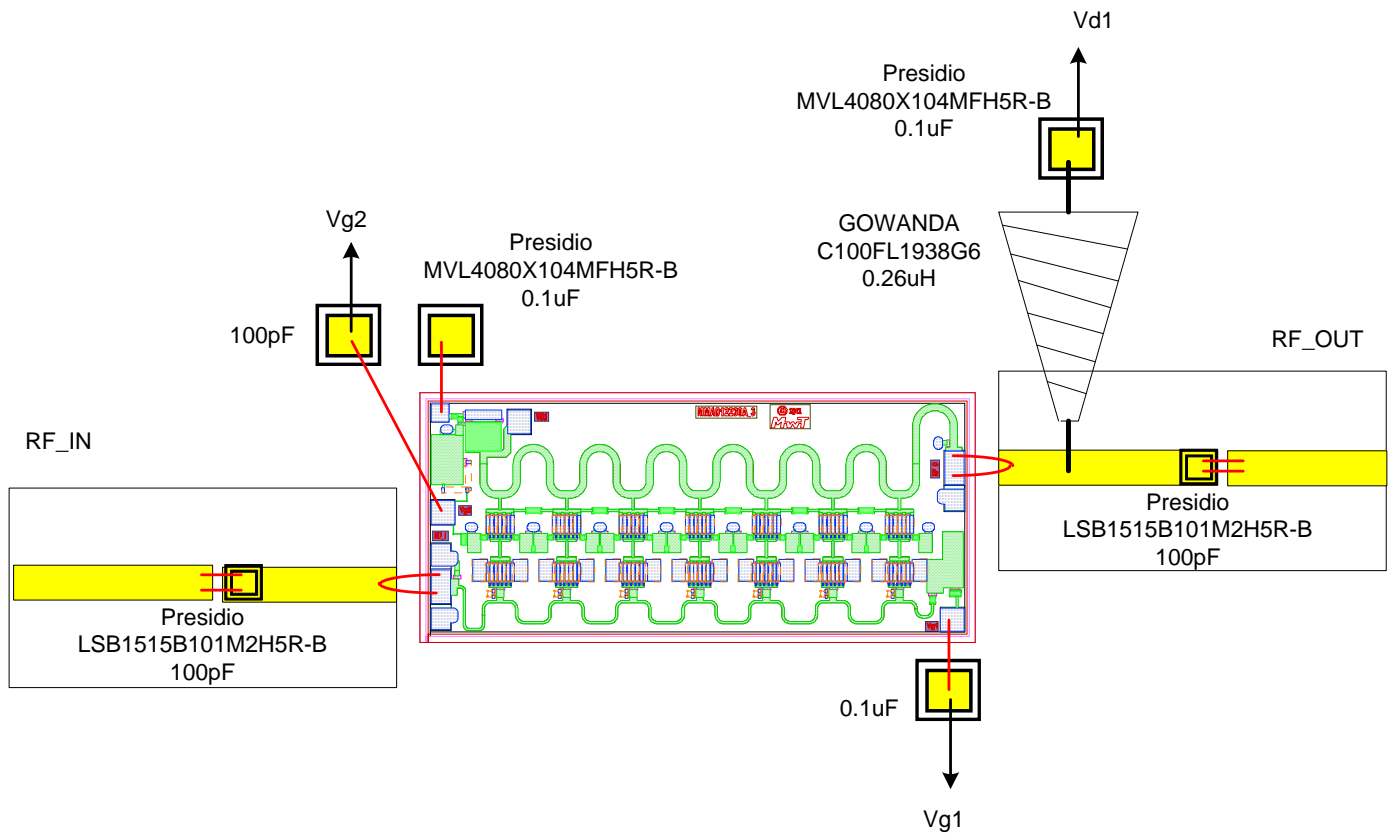
Assembly Diagram
