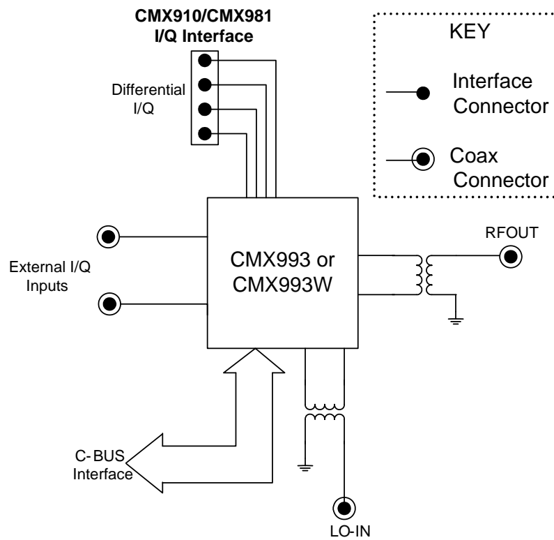
Figure 1 Block Diagram
