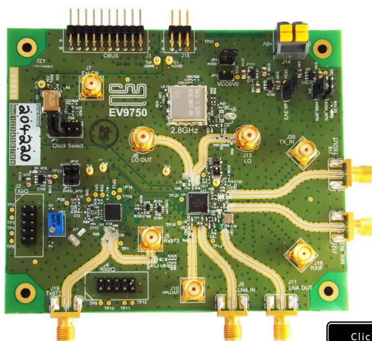
Figure 1 EV9750 board
