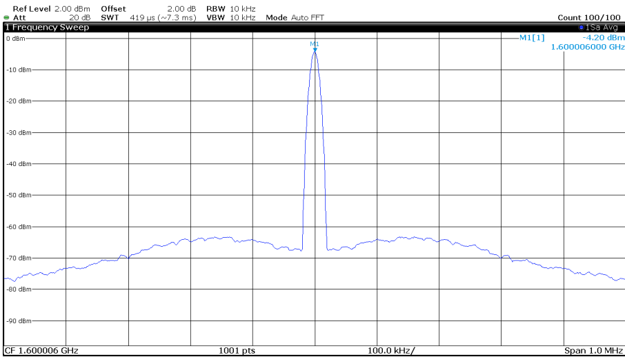
Figure 23 Typical RF VCO output at J8, 1.6GHz, Fractional-N mode using 3.2GHz wide loop filter values, 400µA charge pump current, 38.4MHz comparison frequency
