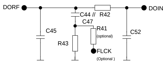
Figure 9 Example External Components – VCO External Loop Filter
