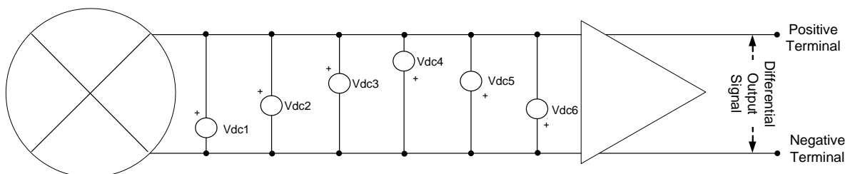
Figure 11 Simplified Schematic DC Offset Correction Circuit
