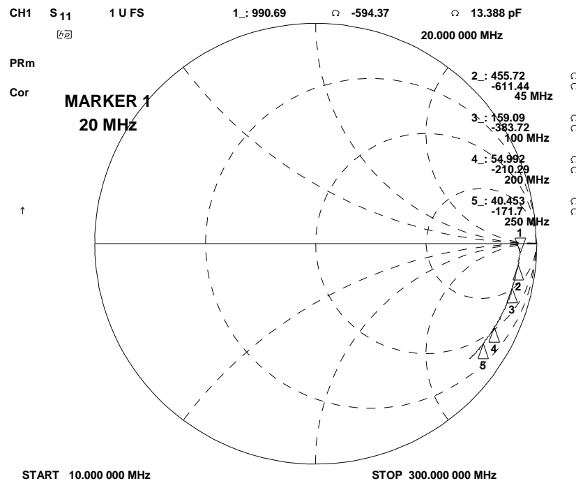
Figure 14 Quadrature Demodulator Input Impedance (10MHz to 300MHz)
