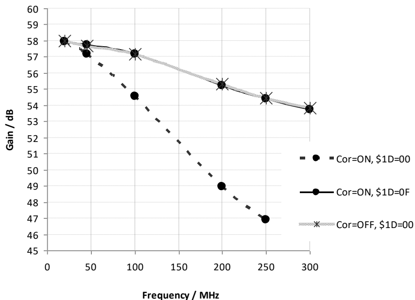
Figure 10 Frequency Response, showing effect of COR bit ($1C, b6) and FREQ bits($1D, b3-b0)
