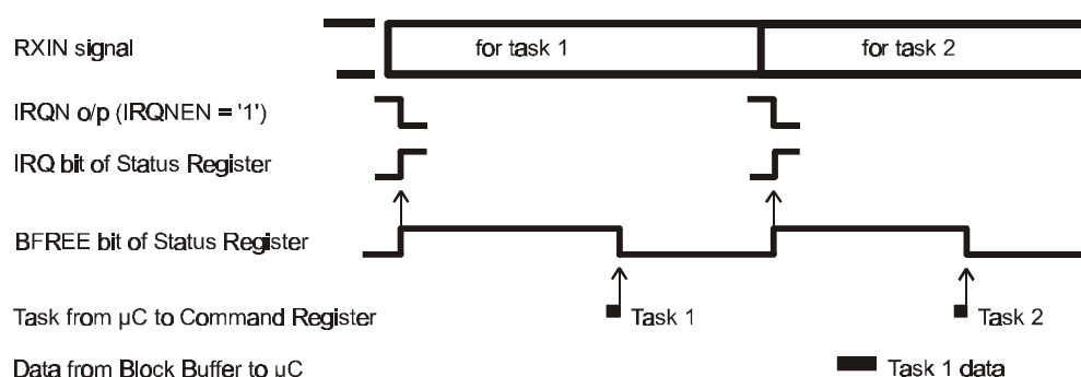
Figure 8 Receive Task Overlapping
