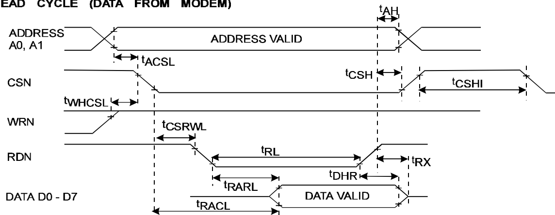
Figure 14 \mu C Parallel Interface Timings
