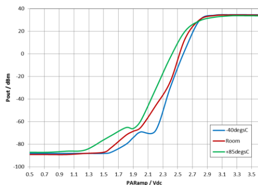
Figure 4 Output power vs. control voltage characteristics and variation with temperature, V_{DD} = 4V , input level = -5dBm
