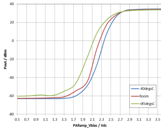
Figure 8 Output power vs. control voltage characteristics variation with temperature, V_{DD} = 4V , input level = -5dBm
