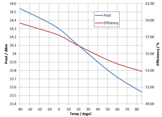
Figure 9 Output power and efficiency variation with temperature, V_{DD} = 4V , input level = -5dBm, V_{PARAMP} = 3.3V
