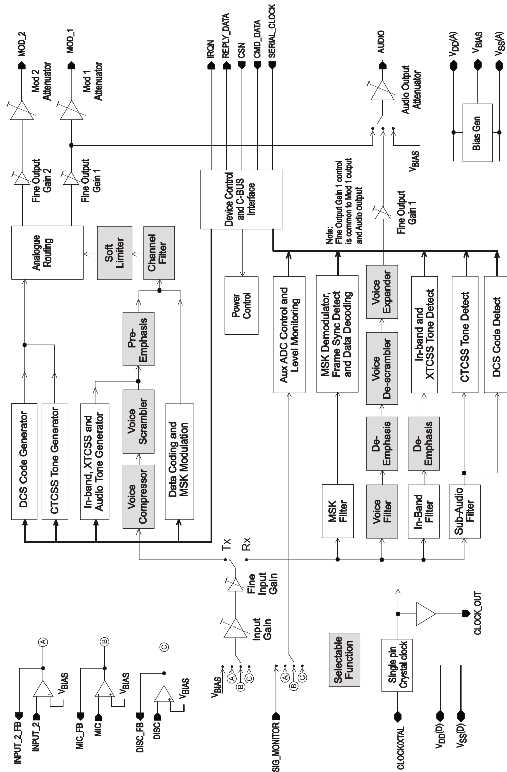
Figure 1 Block Diagram
