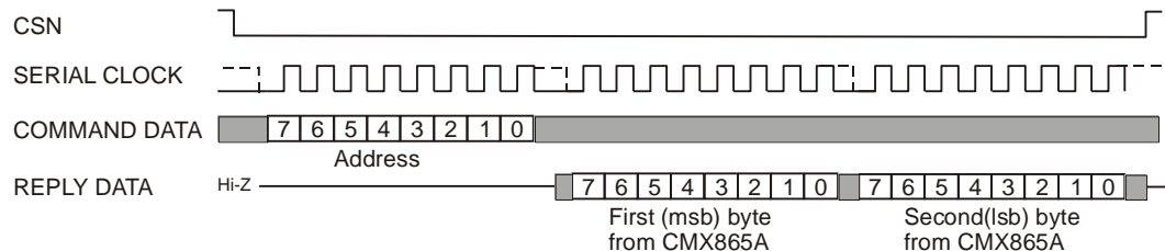
Figure 14 C-BUS Transactions
