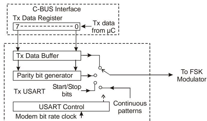
Figure 6 Tx USART
