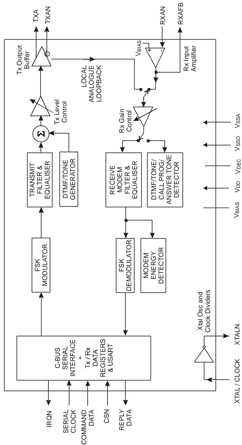
Figure 1 Block Diagram
