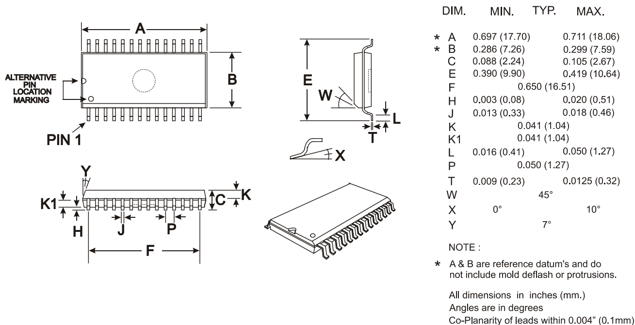
Figure 50: 28-pin SOIC (D1) Mechanical Outline: Order as part no. CMX838D1
