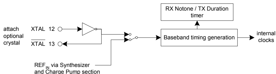
Figure 40: Clock Generation
