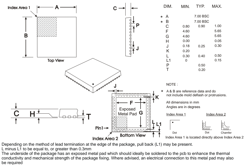
Figure 9 48-pin VQFN Mechanical Outline (Q3)
