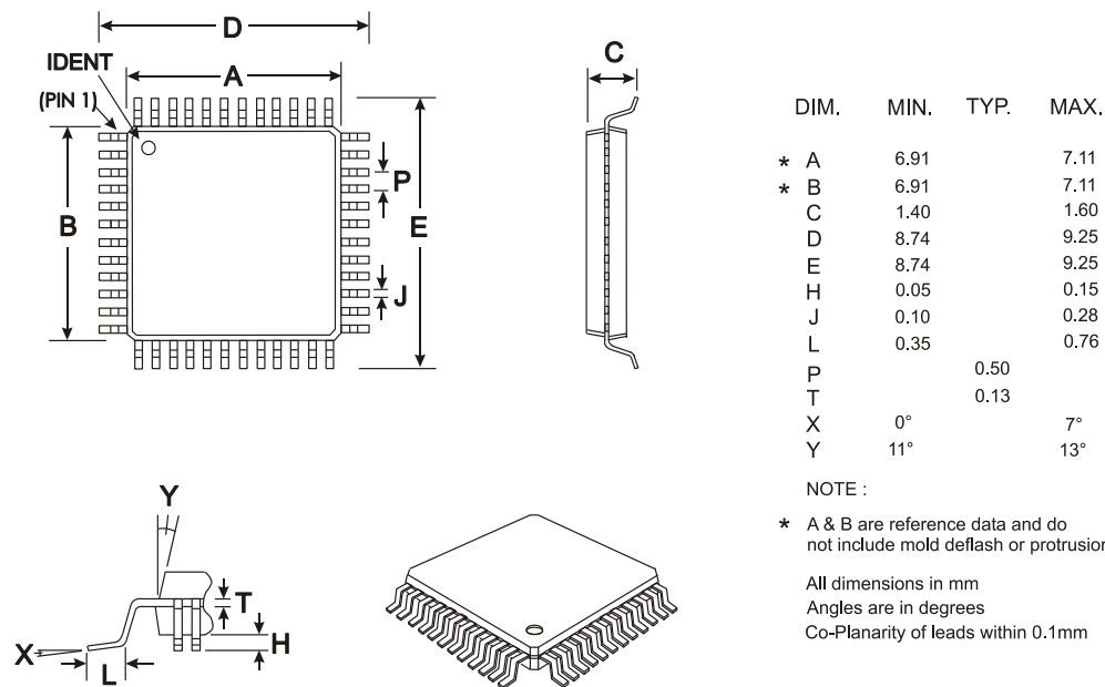
Figure 32 Mechanical Outline of 48-pin LQFP (L4)
