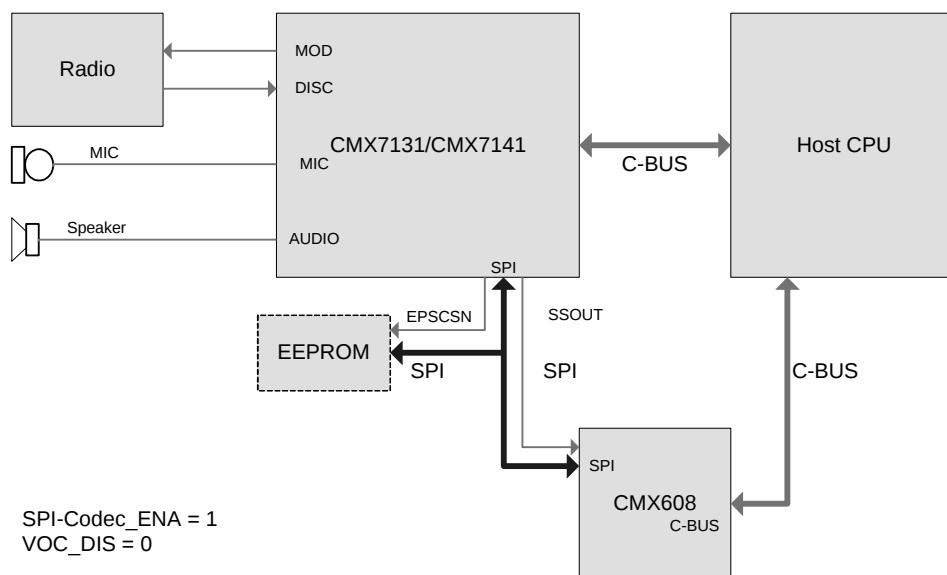
Figure 7 CMX608 Vocoder Connection
