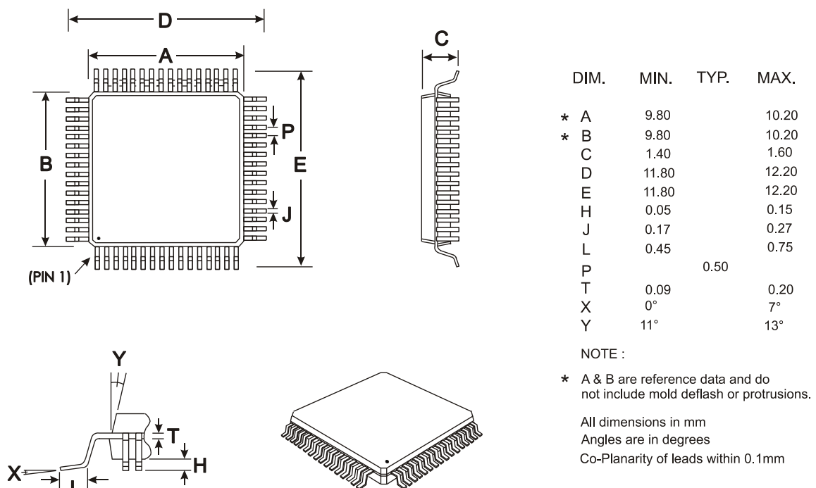
Figure 31 Mechanical Outline of 64-pin LQFP (L9)
