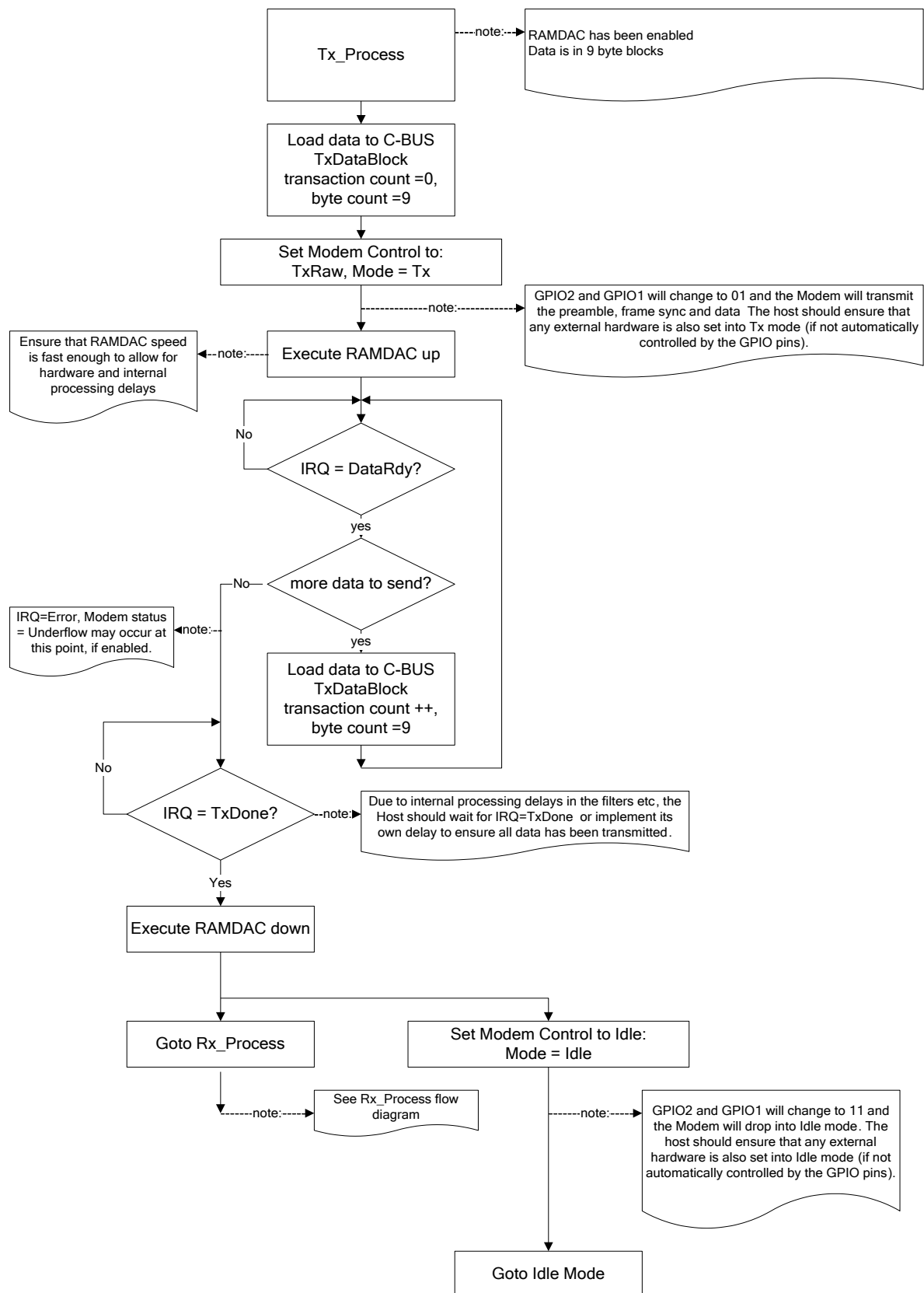
Figure 20 Tx Data Flow (Raw Data Mode)
